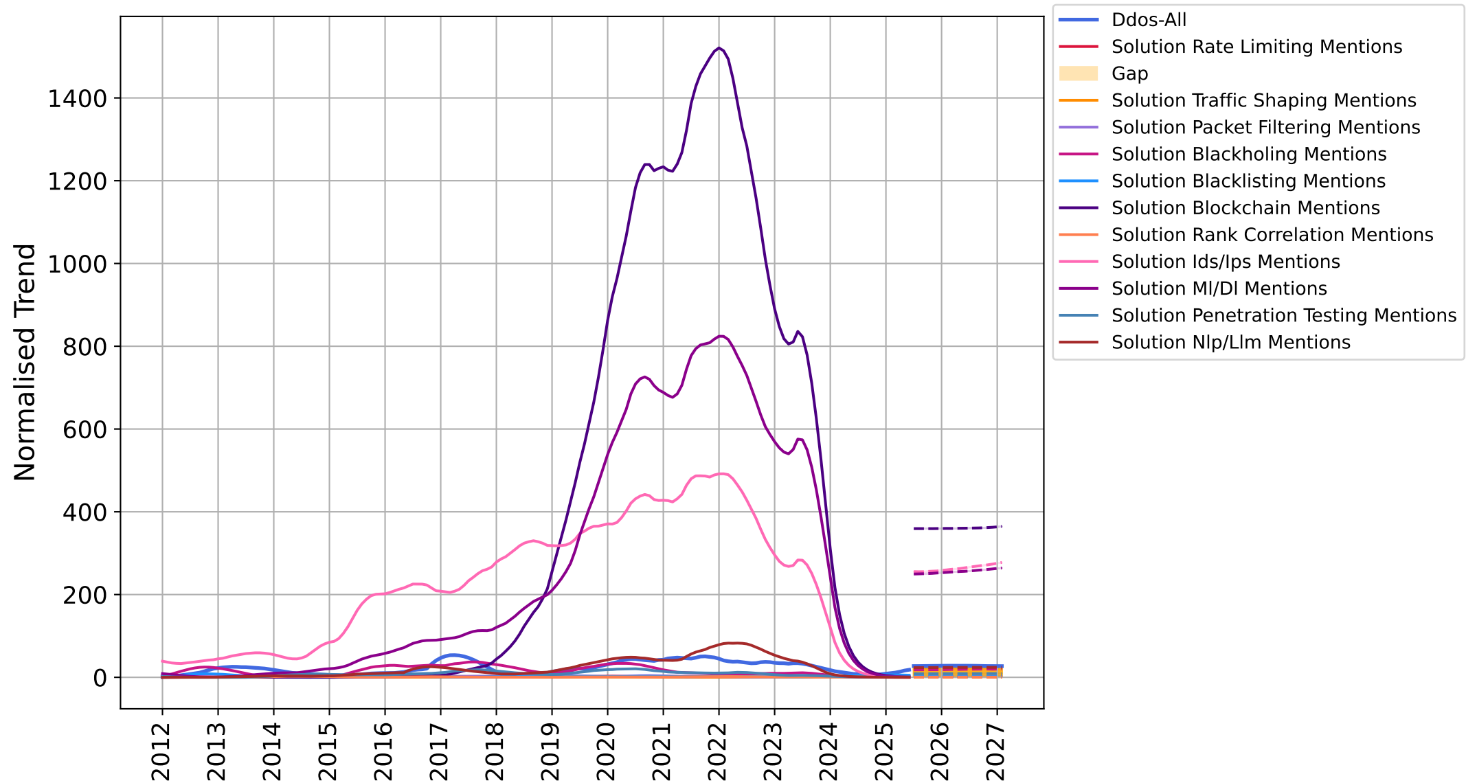
Ddos-All Forecast
